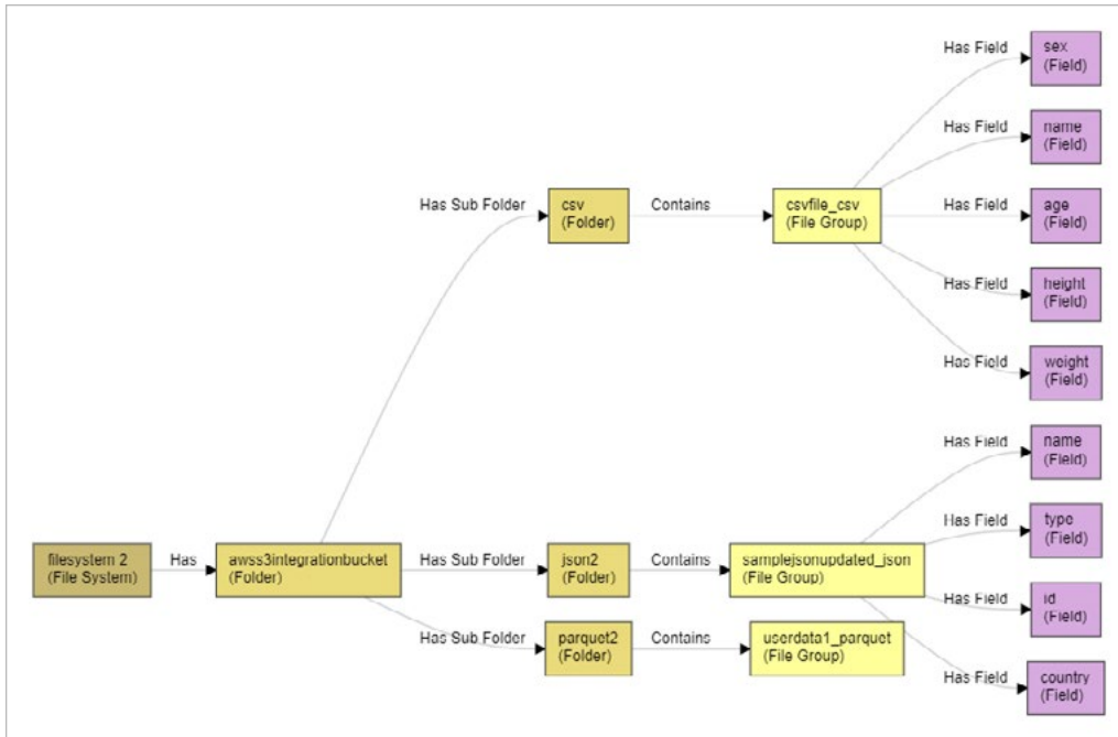
Figure 1: End-to-end traceability of Amazon S3 objects in YourDataConnect
